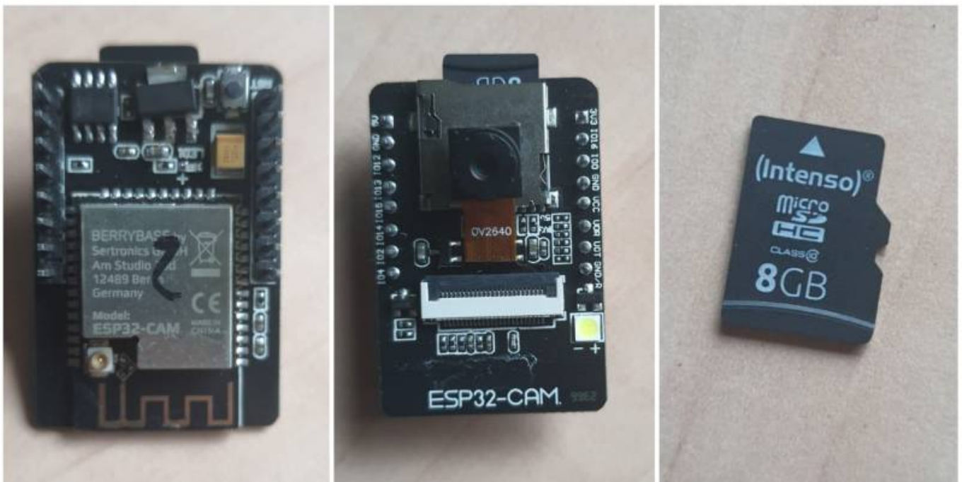
Fig 2. ESP32-Cam AI-Thinker + 8Gb SD Card
