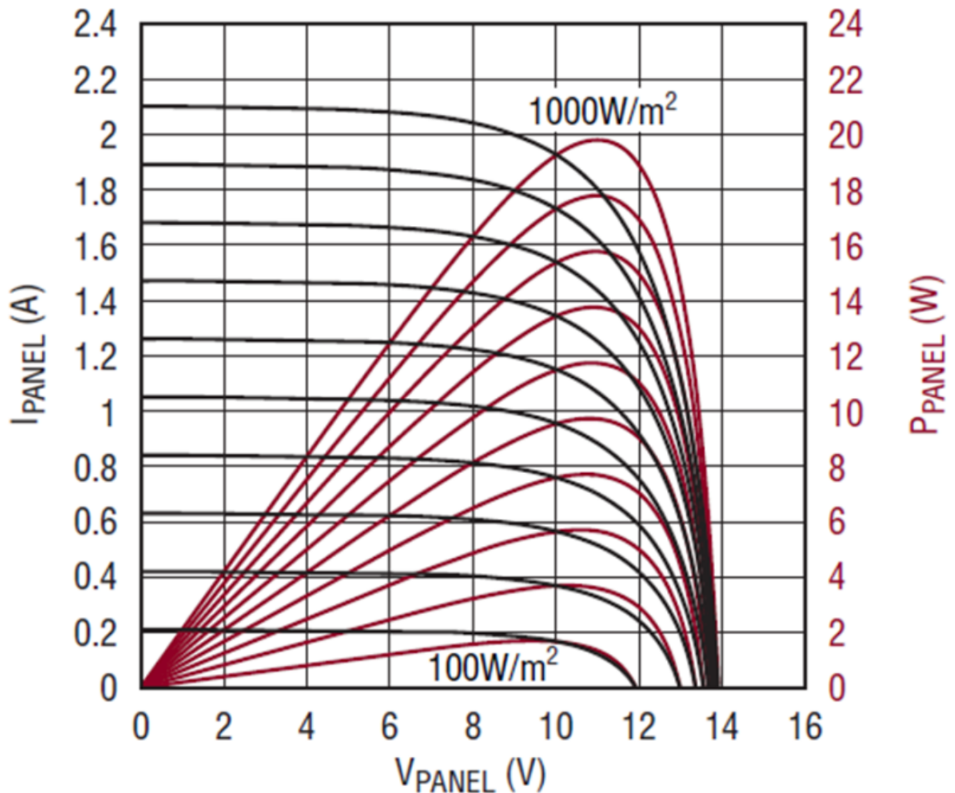
Fig 4. Solar panel module
