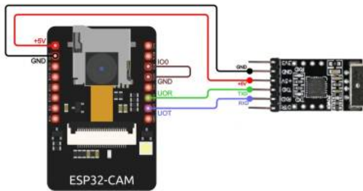
Figure 5. ESP32-CAM and Programmer connection Sketch
