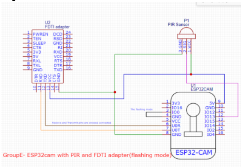
Fig3: Esp32 cam on flashing mode(
