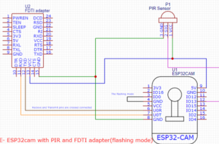
GroupE- ESP32cam with PIR and FTDI adapter(flashing mode)
