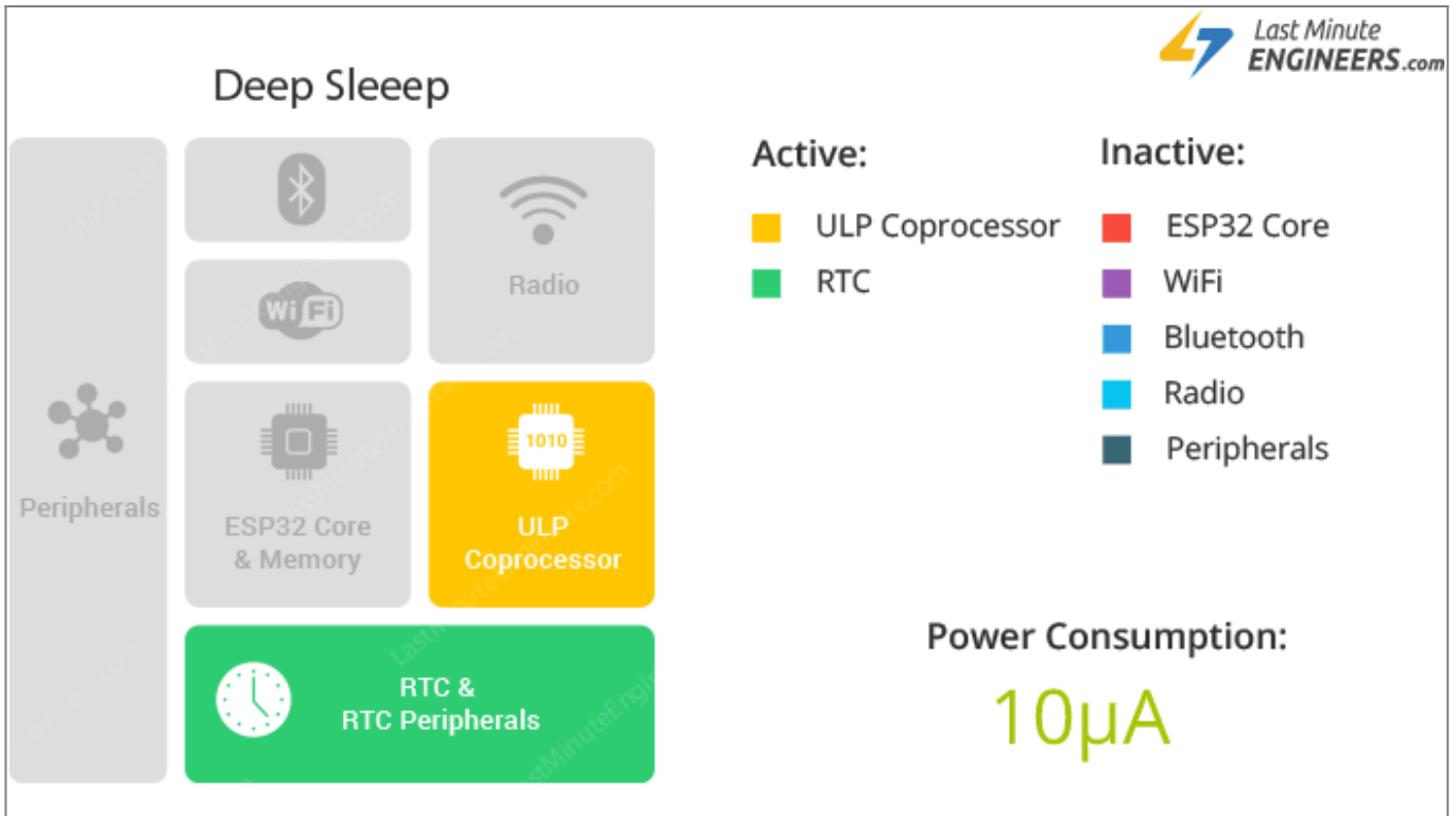
Figure 10. Deep sleep mode
