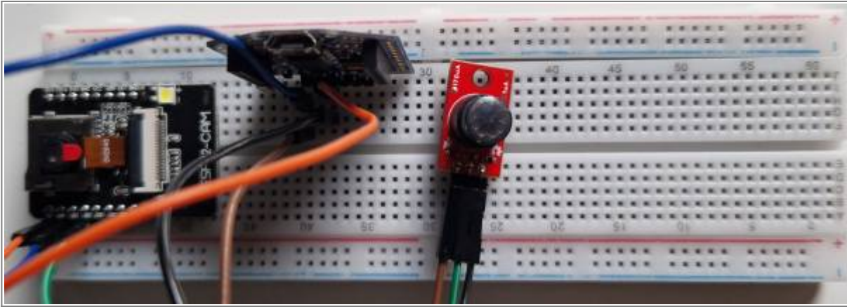
Fig.7: Circuit
