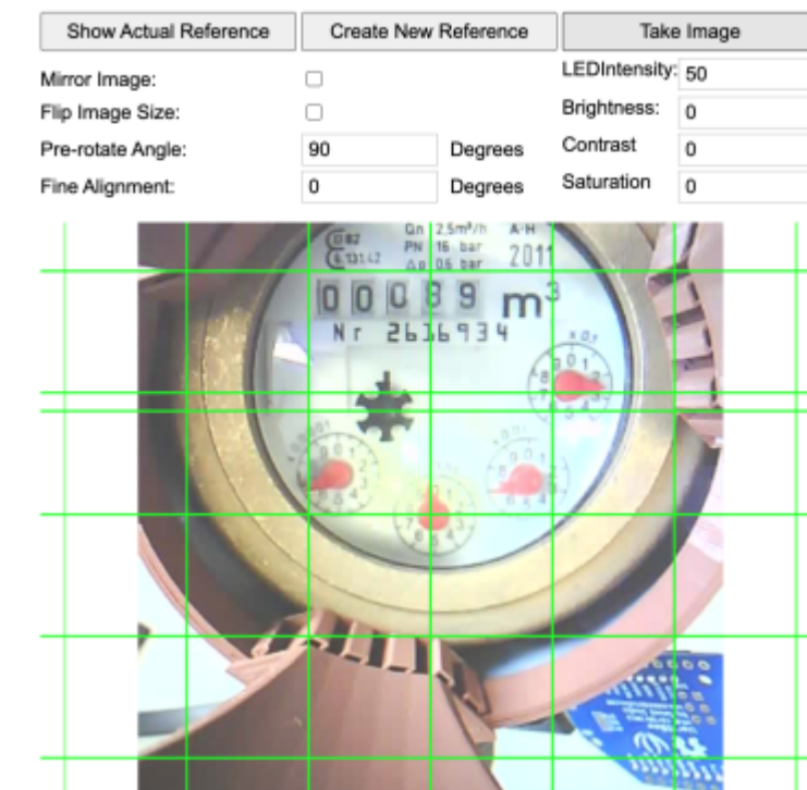
Figure 13: AI-on-the-edge setup webpage
