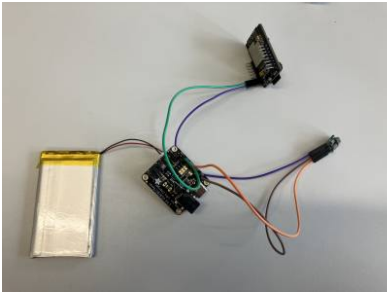
Figure 12: Power supply setup
