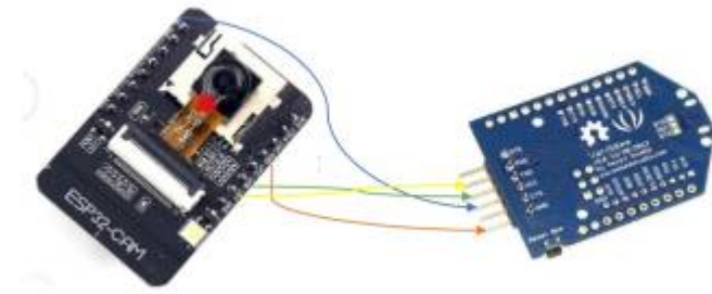
Figure 9: Connection setup of ESP32CAM with UartSBee
