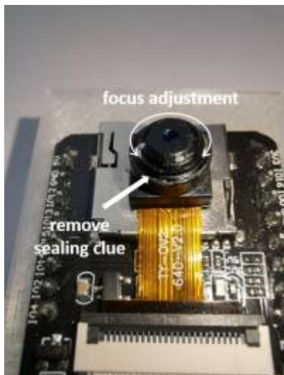
Figure 10: Focus adjustment of the camera
