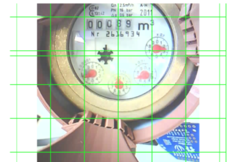
Figure 13: AI-on-the-edge setup webpage
