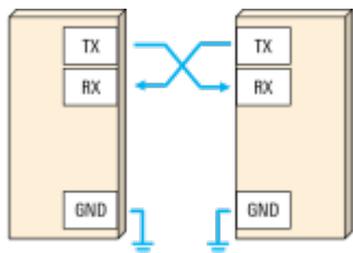
Figure 4: Uart uses two wires between transmitter and receiver to transmit and receive in both directions.
