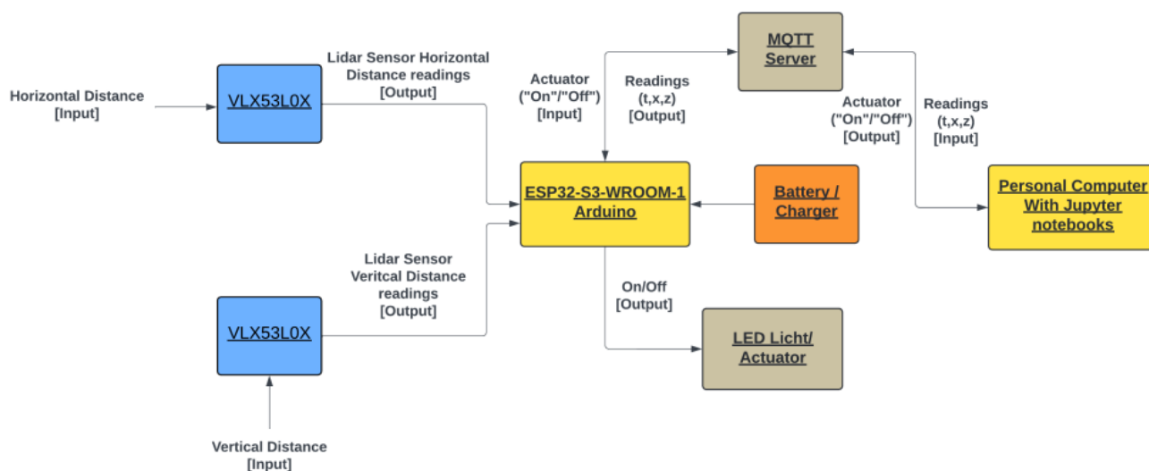
Figure 1: Project Layout
