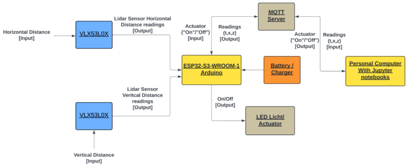
Figure 1: Project Layout
