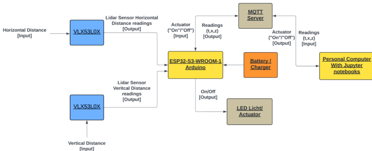
Figure 1: Project Layout
