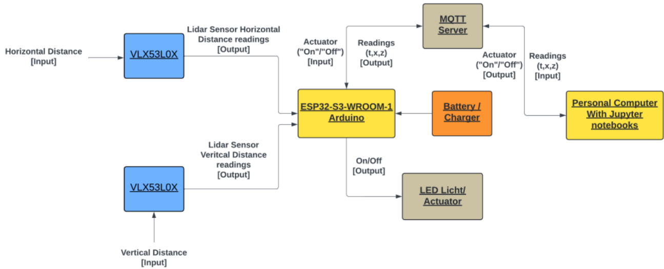
Fig. 1: Project Layout
