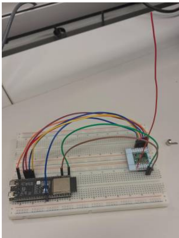
Fig. 7: Second prototype IMU data Transmitter Fig. 7: Second prototype data Receiver
