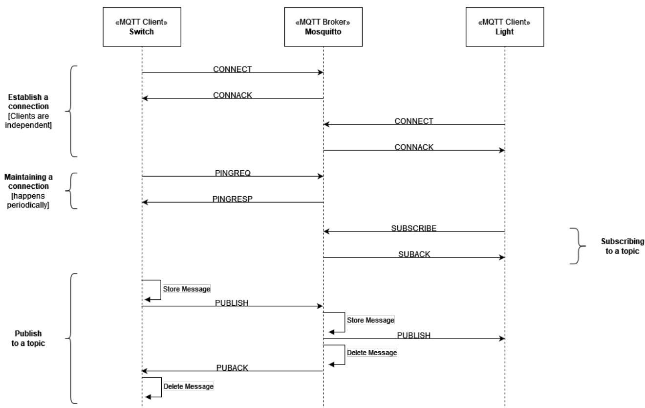
MQTT Full Sequence Example [QOS 1]
