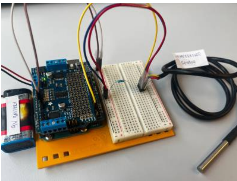
Figure 2. DS18B20 digital temperature sensor wired to digital pin D2, with a 4.7kΩ pull-up resistor between data and VCC
