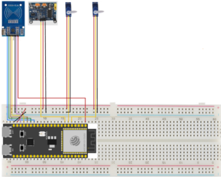
Fig. 1: Wiring model
