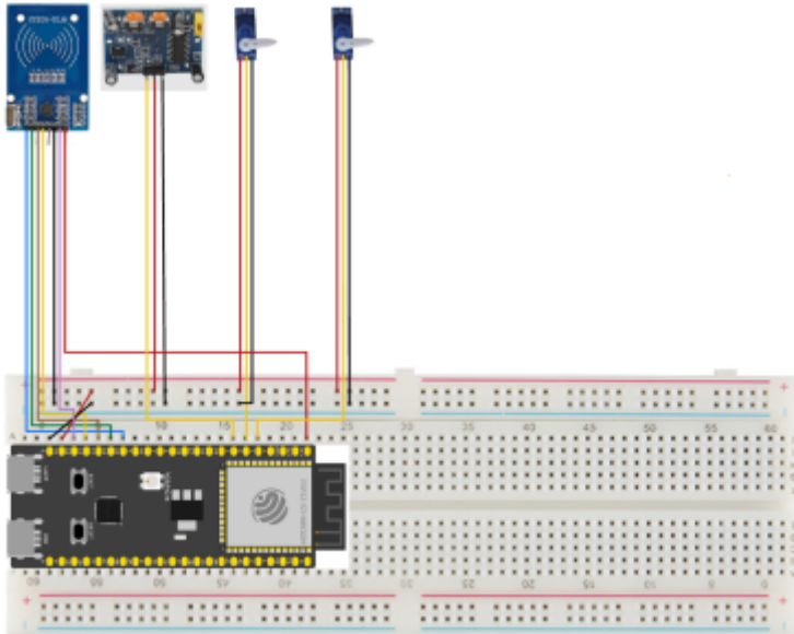
Fig. 1: Wiring model
