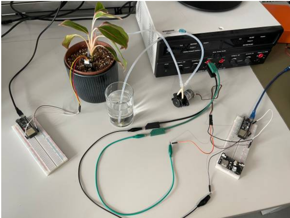
}} Figure 1. Automated Plant Watering System Prototype
