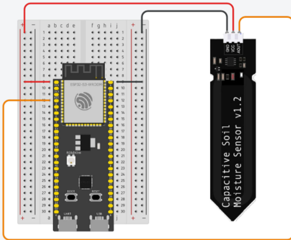
Figure 2. Schematic Diagram of Sensor Setup (designed by Deniz-Zeynep Adem)
