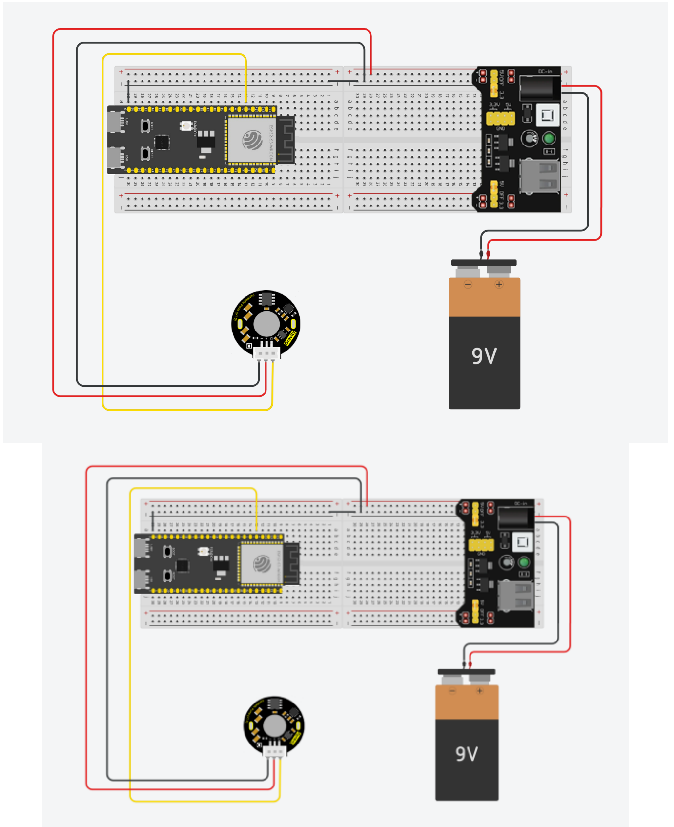
Figure 3. Schematic Diagram of Pump Setup (designed by Deniz-Zeynep Adem)
