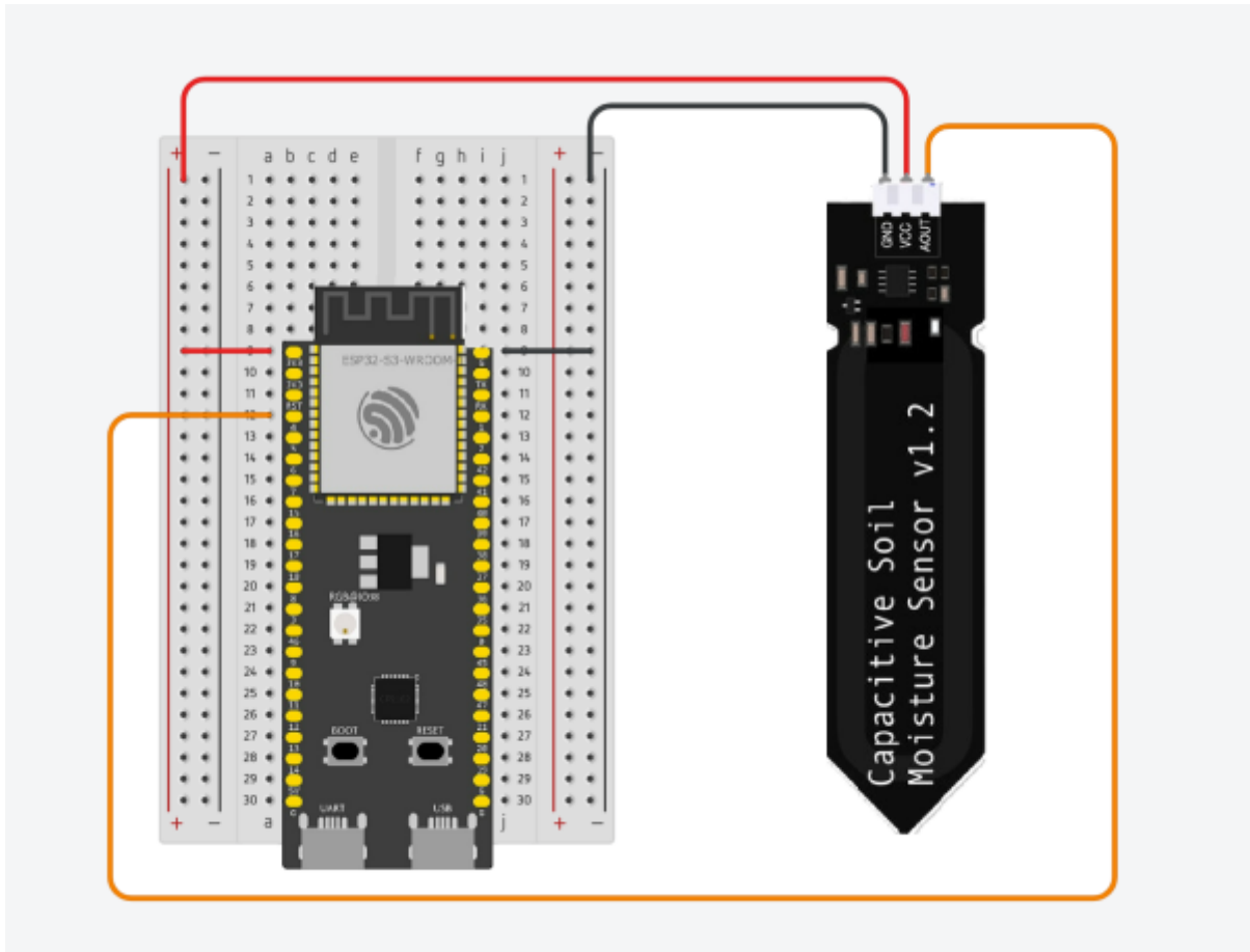
Figure 2. Schematic Diagram of Sensor Setup (designed by Deniz-Zeynep Adem)
