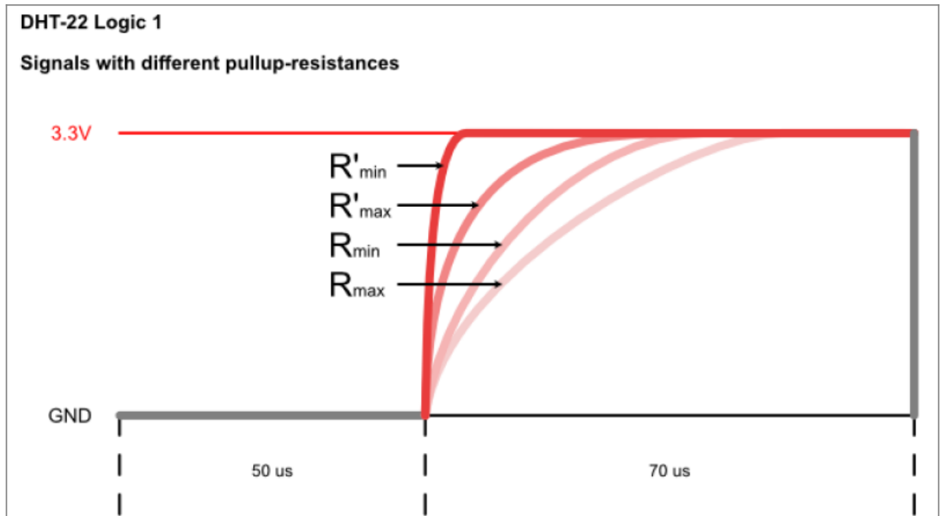
Figure 3 Schematic of how different pullup resistances affect the voltage-time-curve of high voltage level pulses when the wire length is high.
