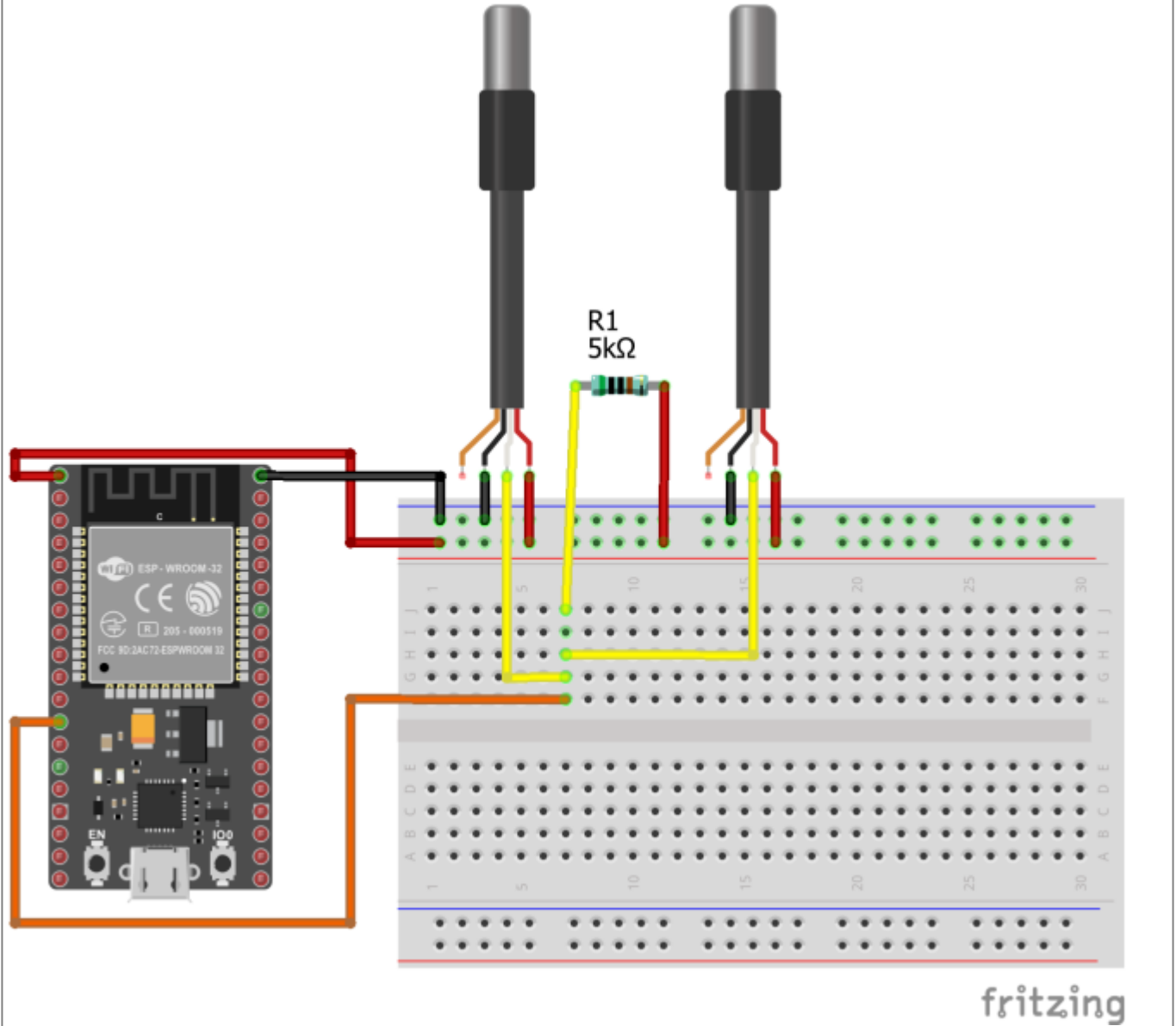
Figure 5 ESP32 connected to two DS18B20s, here the DS18B20s have 4 pins, white is the data bus, orange is not used.
