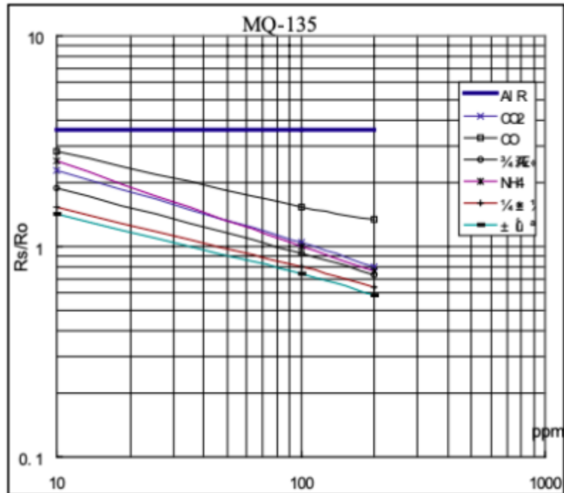
Figure 8: Calibration graph for Mq-135
