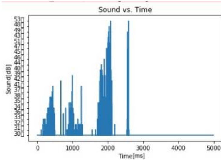
Figure 12: Screenshot of the sound intensity level in decibel using Python . Location: Moerserstraße, Kamp-Lintfort
