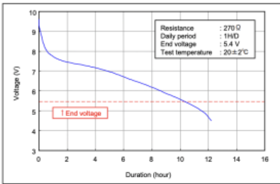
■ Typical Discharge Curve 6F22
