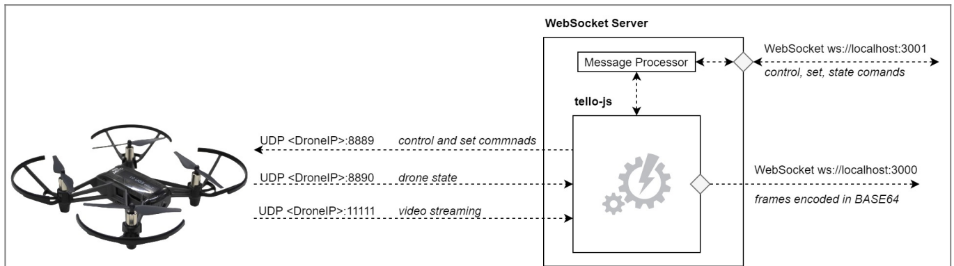
Communication diagram to control Tello drone
