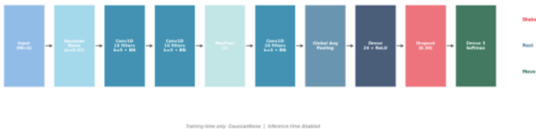
Figure 21 1D-CNN model architecture (v2). Input: (96x6). Output: [move_prob, rest_prob, shake_prob].
