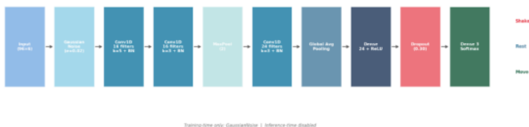
Figure 21 1D-CNN model architecture (v2). Input: (96 \times 6) . Output: [move_prob, rest_prob, shake_prob].
