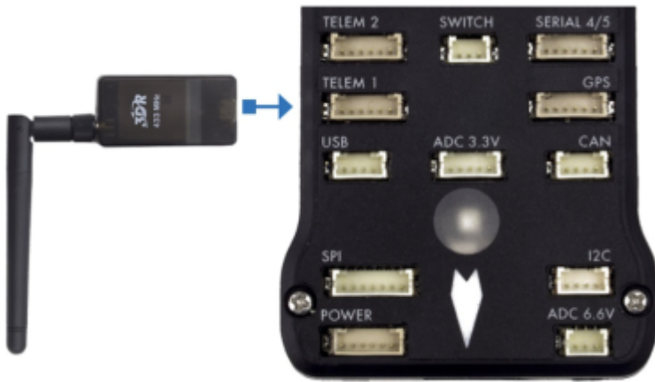
Figure 7.7 Telemetry radio to flight controller
