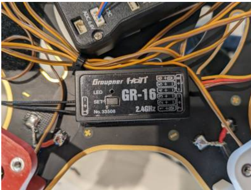
Figure 7.6.2 Radio control
