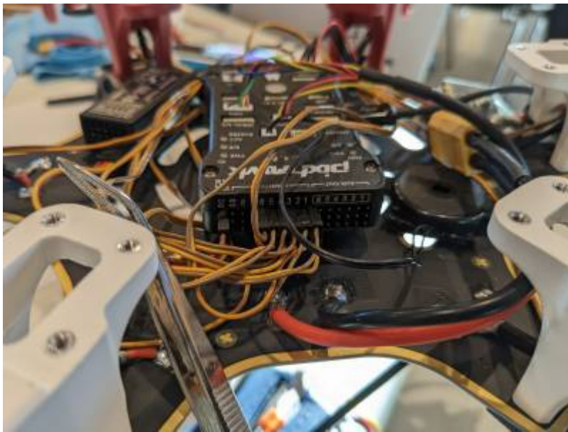
Figure 7.8 Connecting ESCs to the flight controller
