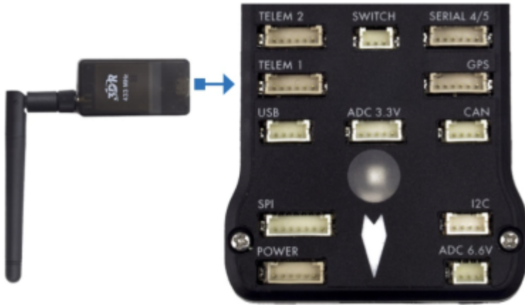
Figure 7.7 Telemetry radio to flight controller
