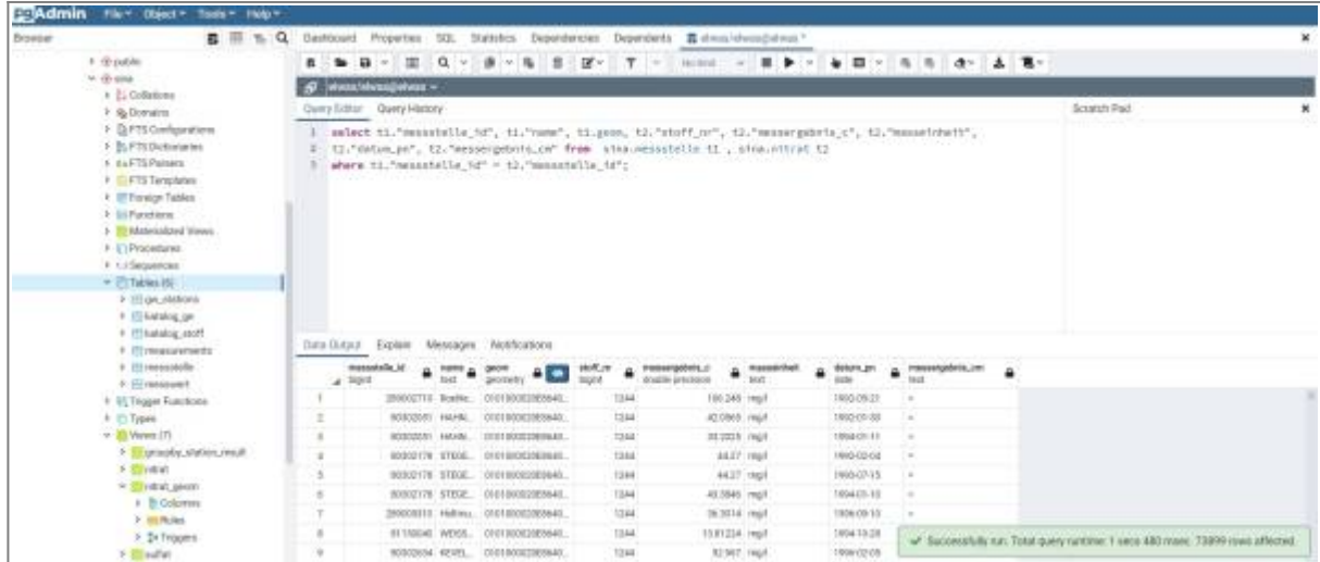
Image 13- Merge tables
