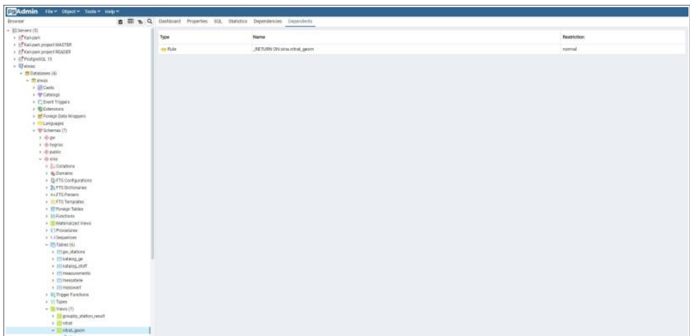
image 6- PGAdmin
